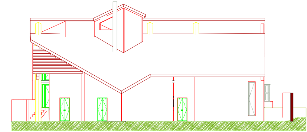
south elevation
